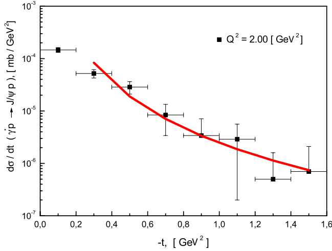
FIG. 5. Angular dependence of the elastic cross sections of exclusive J/\psi -meson electroproduction. Experimental data are taken from [22]. Theoretical curve corresponds to Eqs. (9) and (10).
